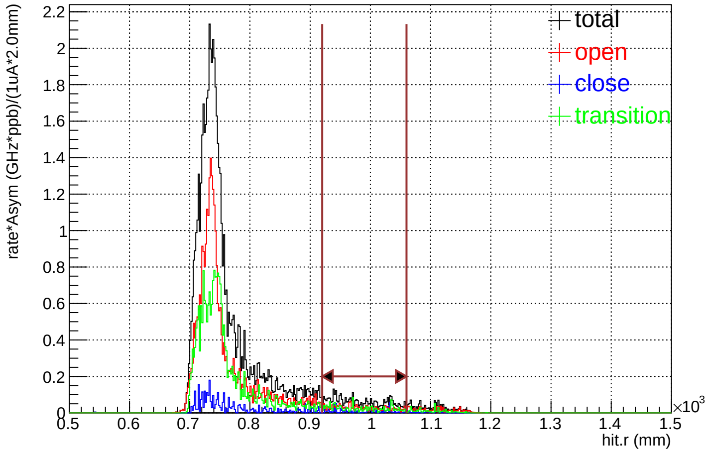
Radial (EP_el) distribution on ring 5 (rate*Asym weighted)
