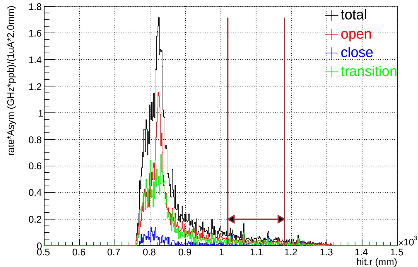
Radial (EP_el) distribution on sm (rate*Asym weighted)
