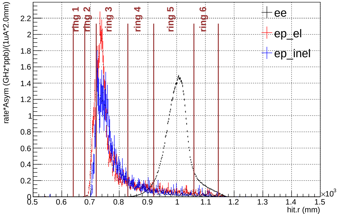
Radial distribution on ring 5 (rate*Asym weighted)
