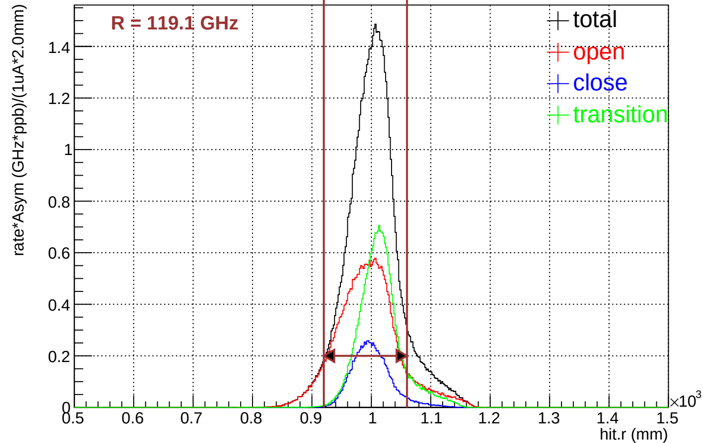
Radial (EE) distribution on ring 5 (rate*Asym weighted)
