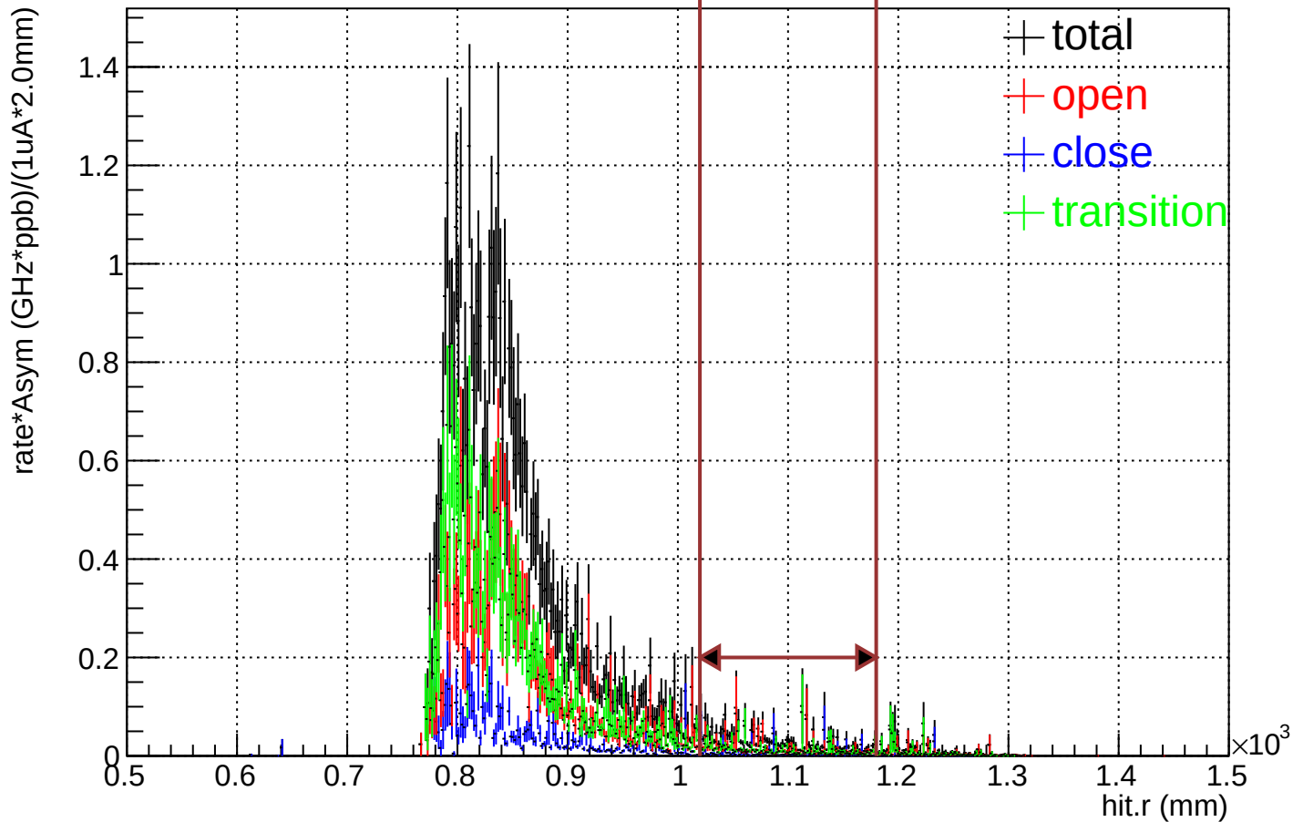
Radial (EP_inel) distribution on sm (rate*Asym weighted)
