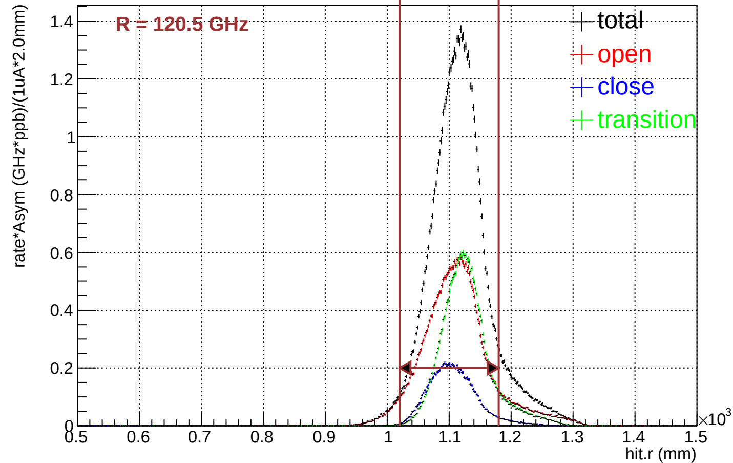
Radial (EE) distribution on sm (rate*Asym weighted)
