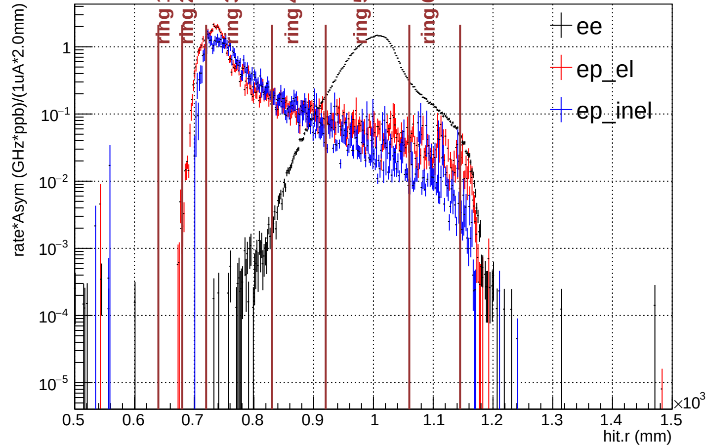
Radial distribution on ring 5 (rate*Asym weighted)
