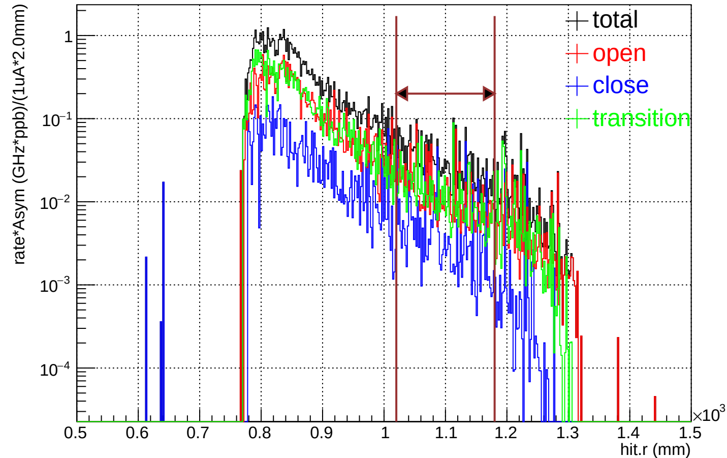
Radial (EP_inel) distribution on sm (rate*Asym weighted)
