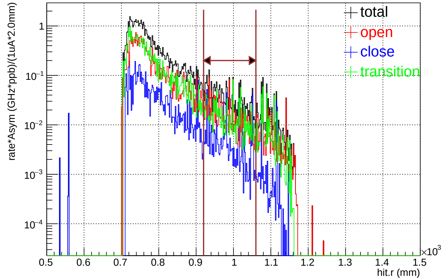
Radial (EP_inel) distribution on ring 5 (rate*Asym weighted)
