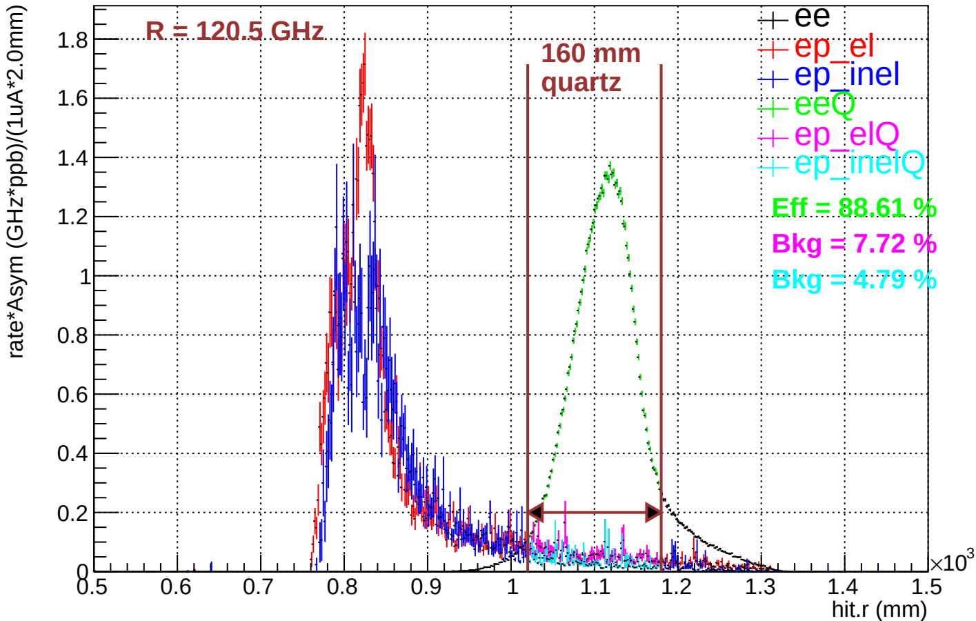
Radial distribution on sm det (rate*Asym weighted)
