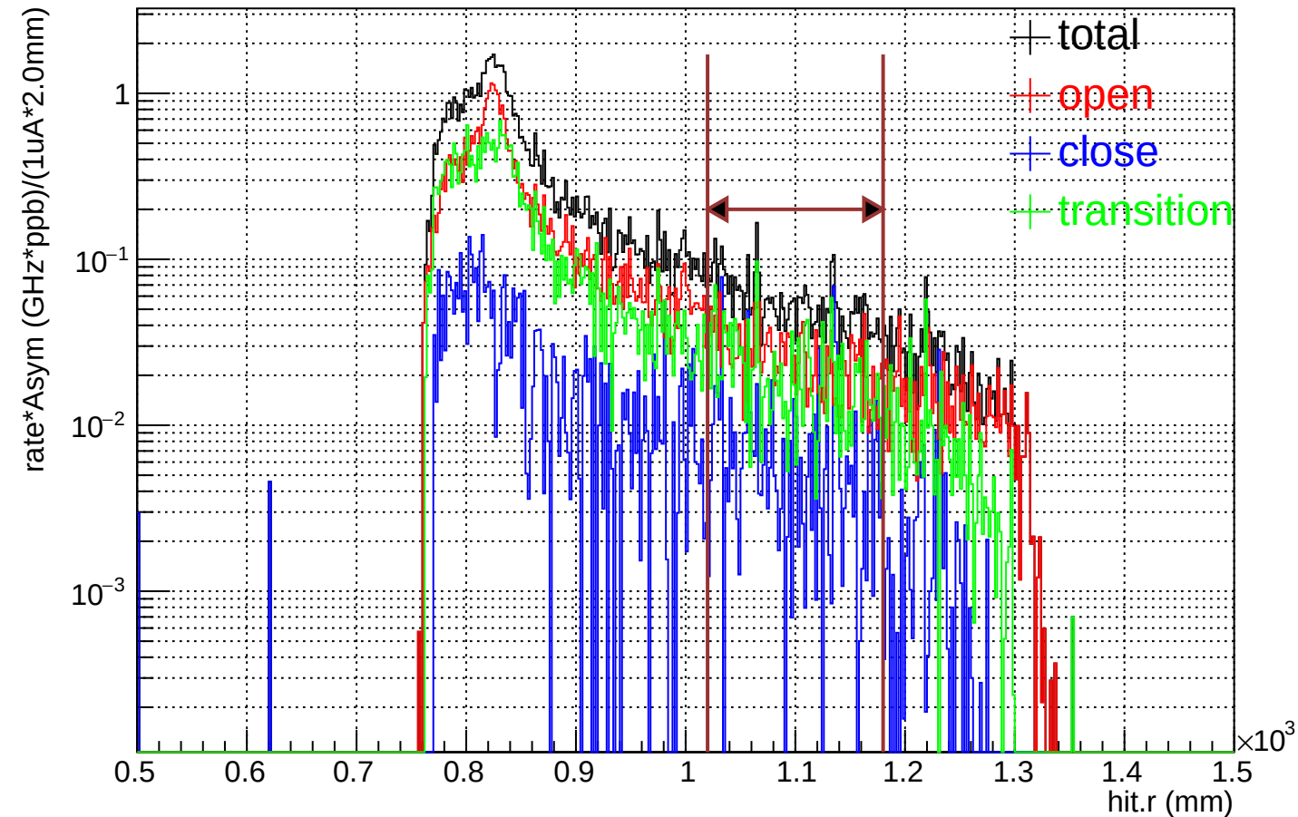
Radial (EP_el) distribution on sm (rate*Asym weighted)
