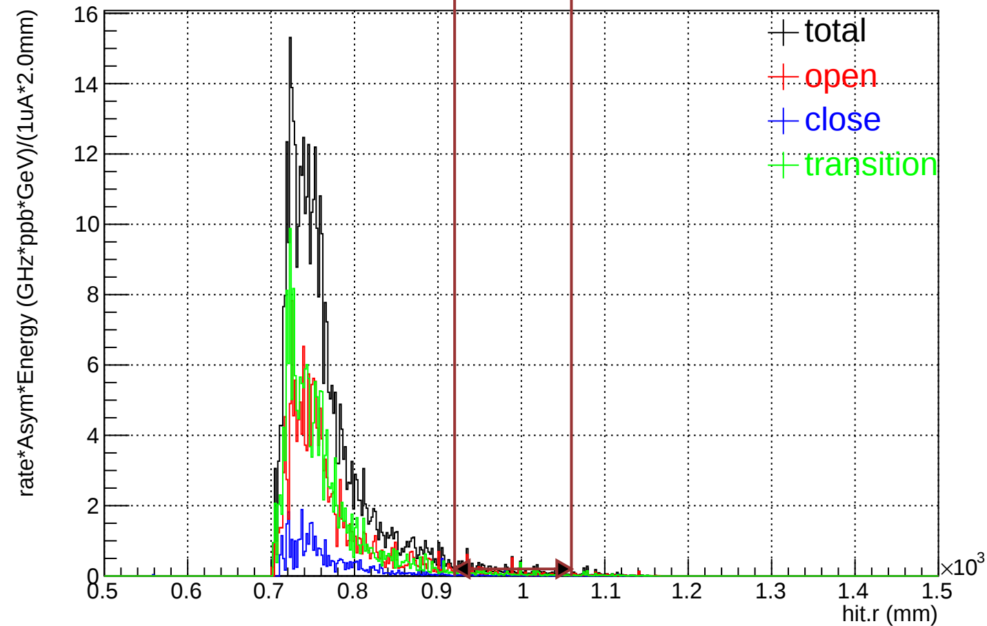
Radial (EP_inel) distribution on ring 5 (rate*Asym*Energy weighted)
