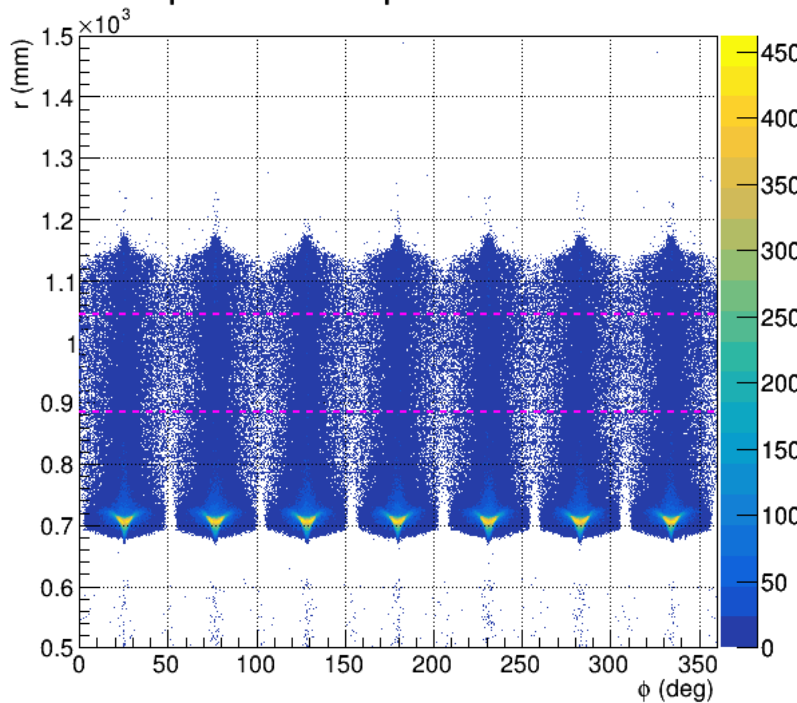
ep-el radial vs phi on main det
