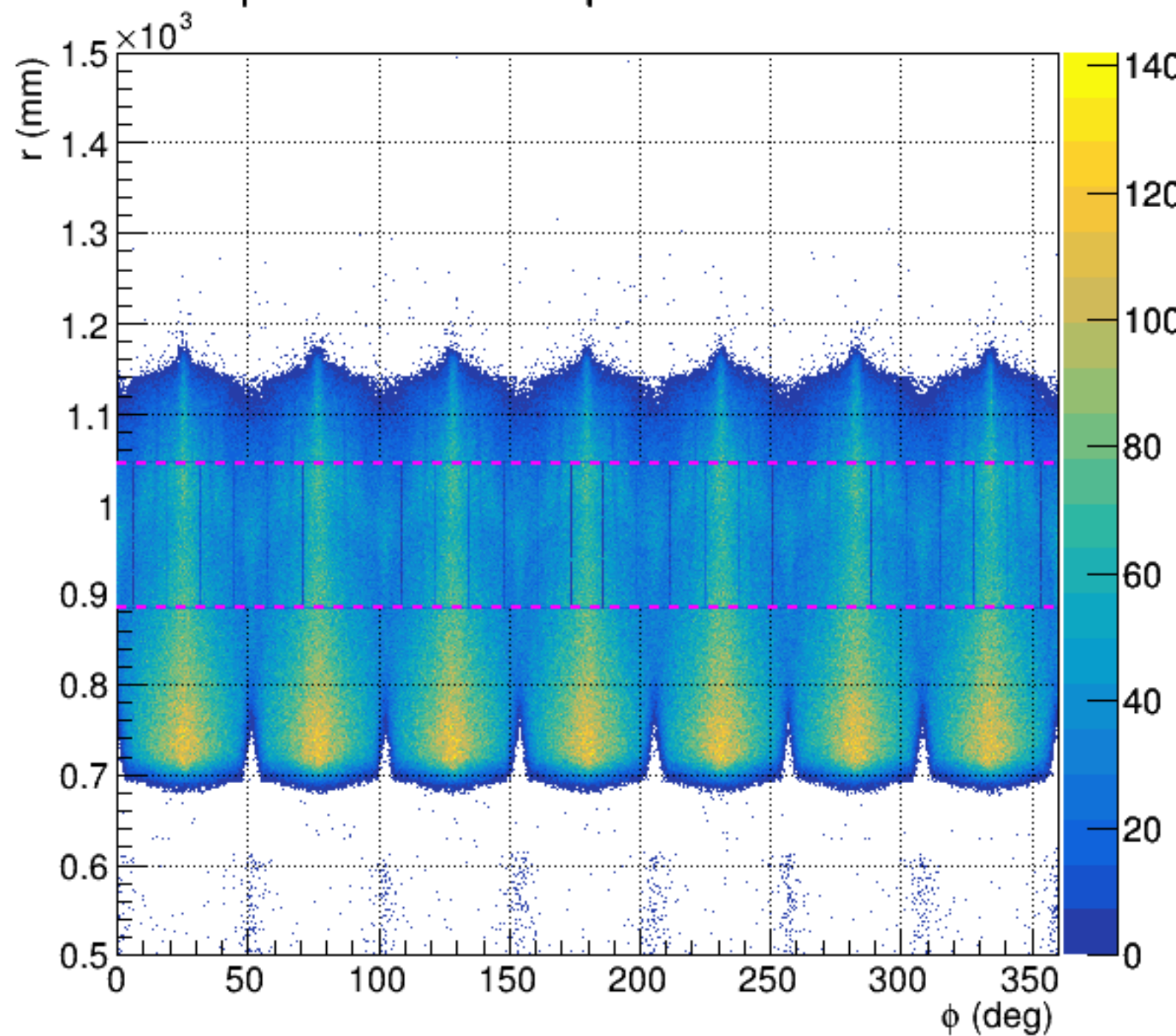
ep-inel radial vs phi on main det
