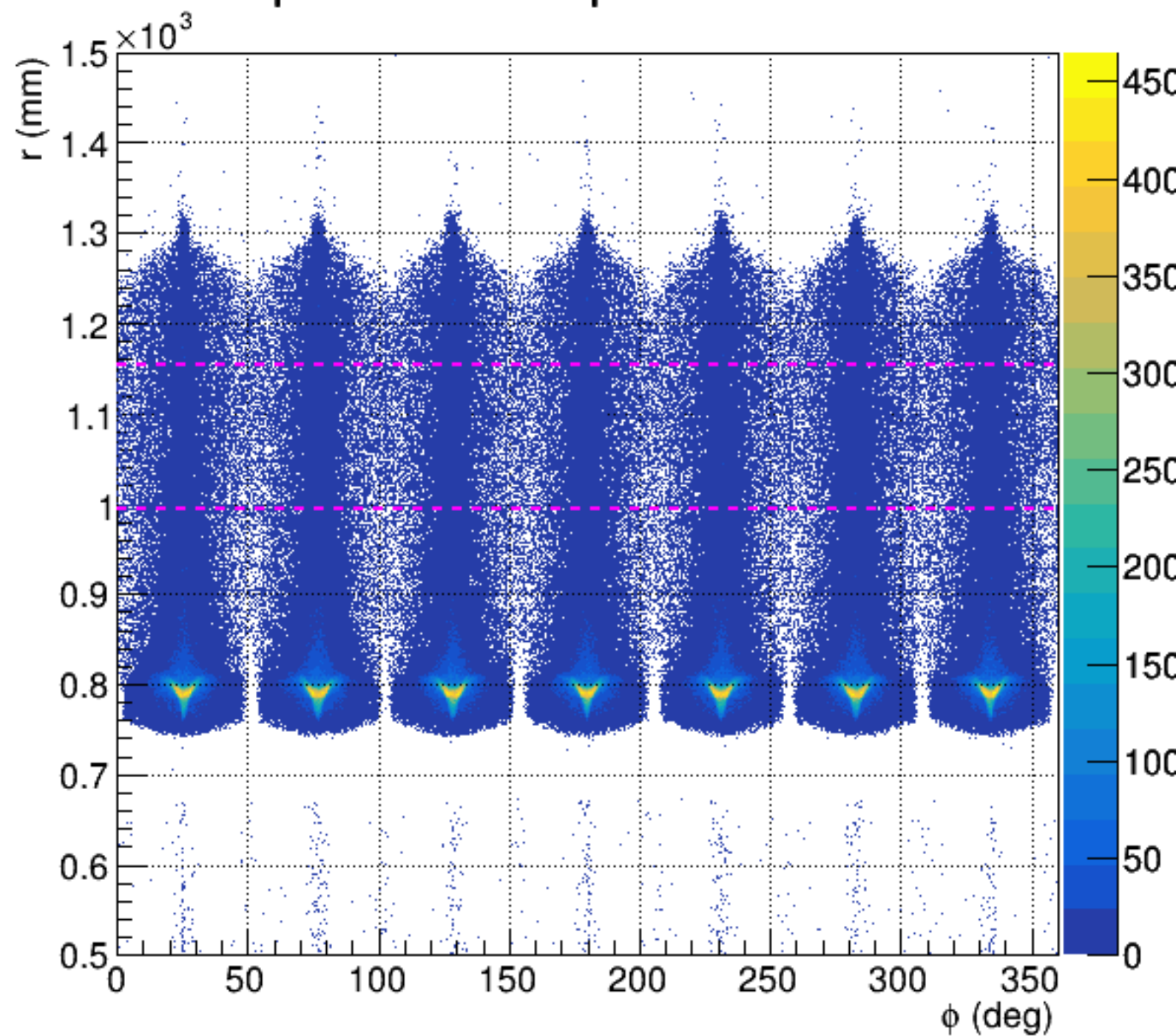
ep-el radial vs phi on sm det
