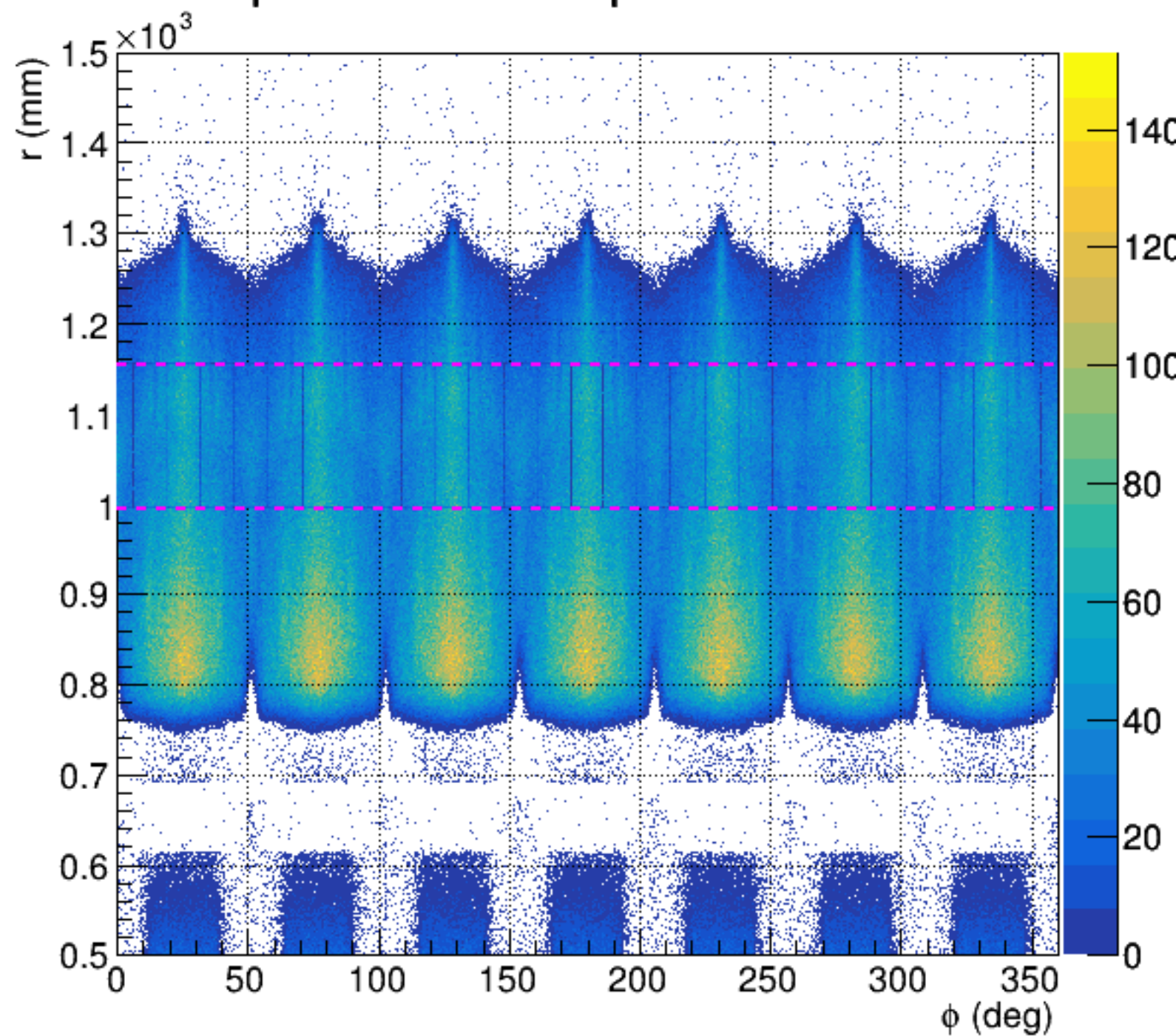
ep-inel radial vs phi on sm det
