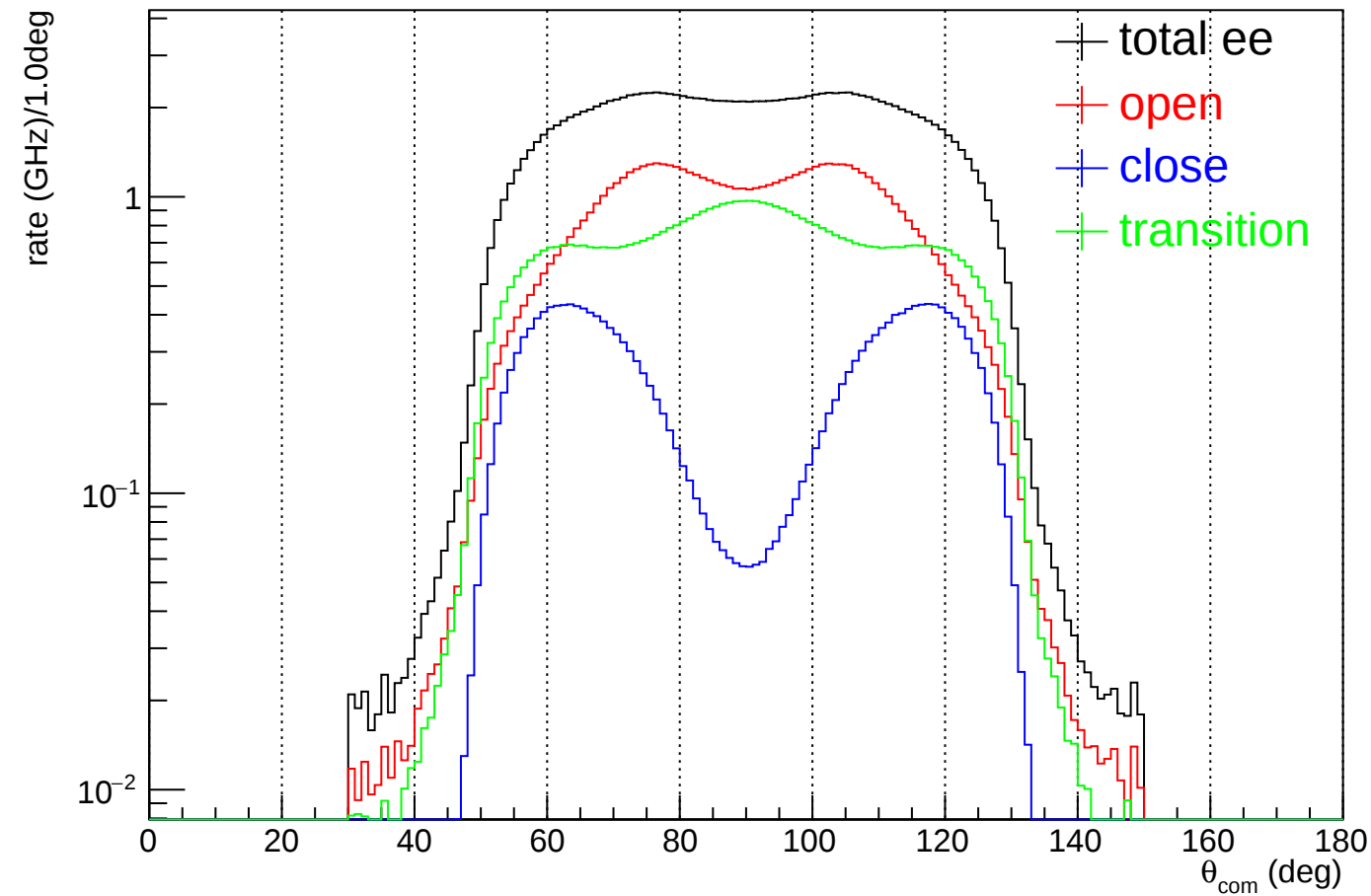
\theta_{\text{com}} distributions (rate weighted)
