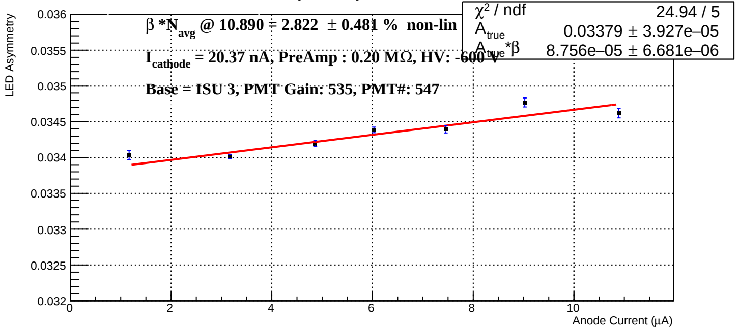
LED Asymmetry vs Anode Current
