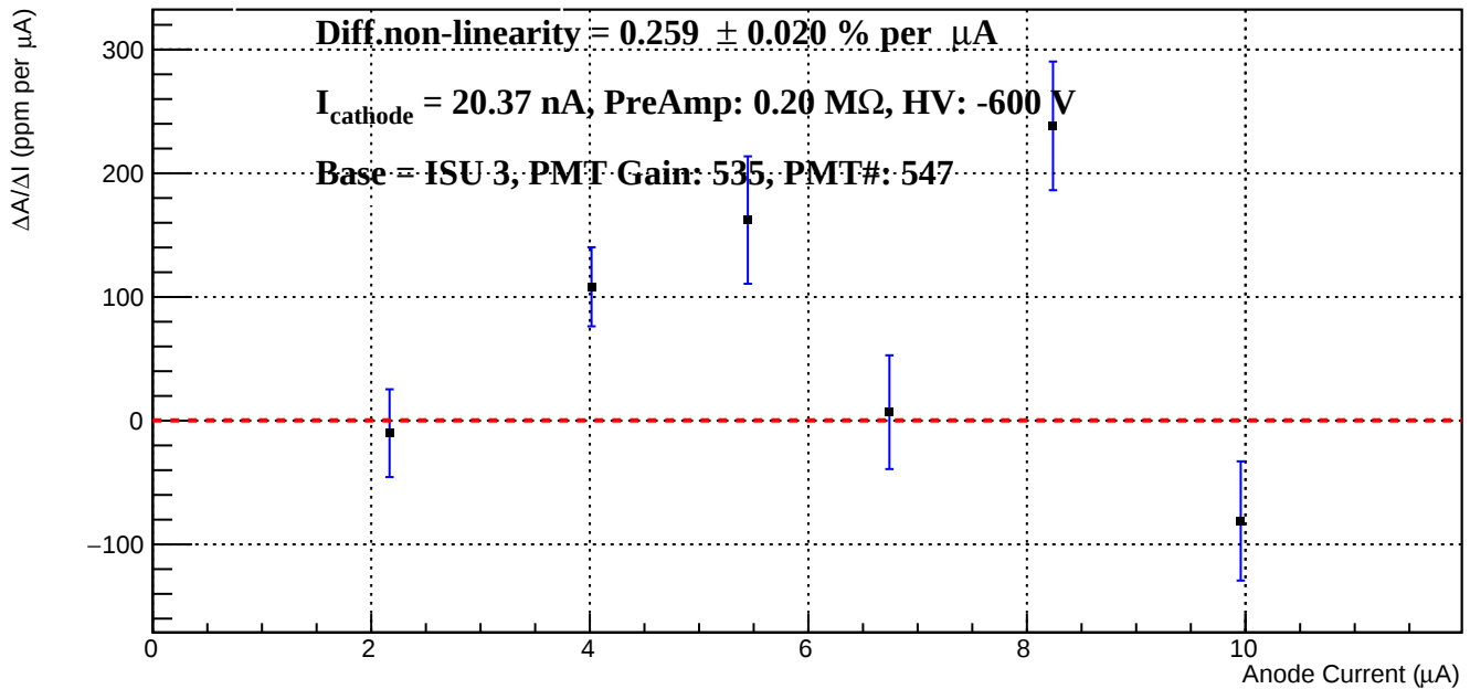
Differential Non-linearity vs Anode Current
