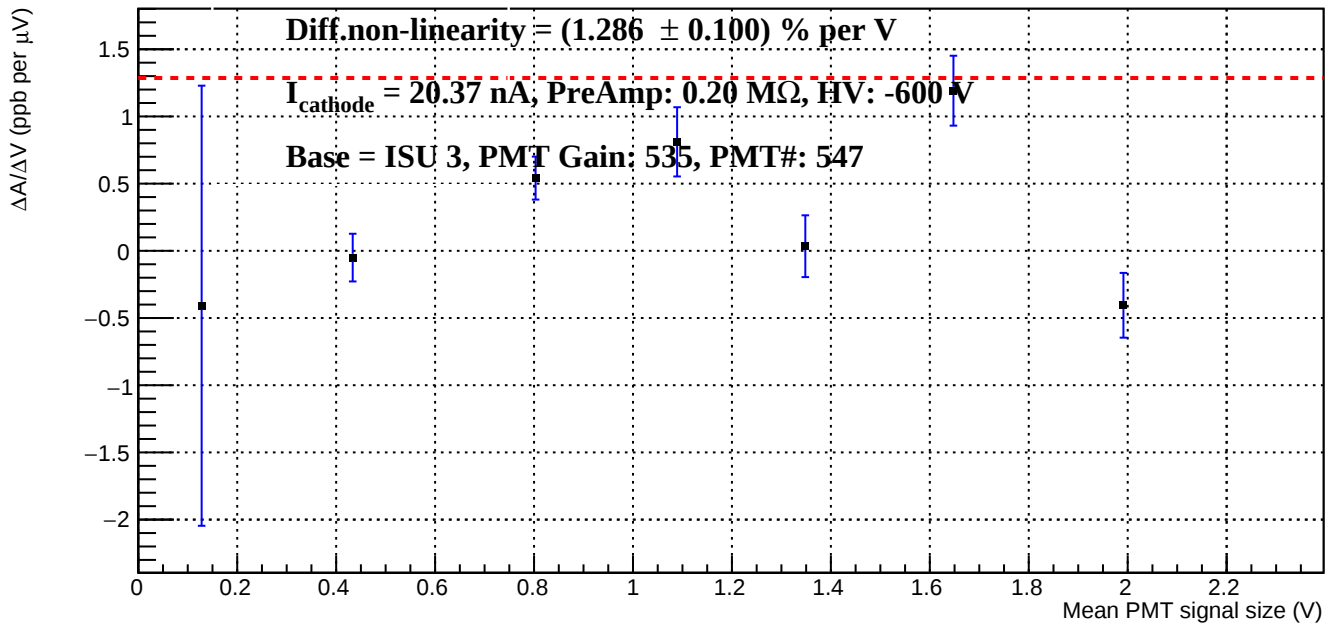
Differential Non-linearity vs Mean PMT signal size
