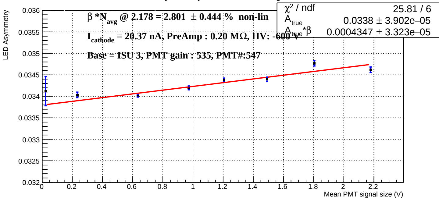
LED Asymmetry vs Mean PMT signal size
